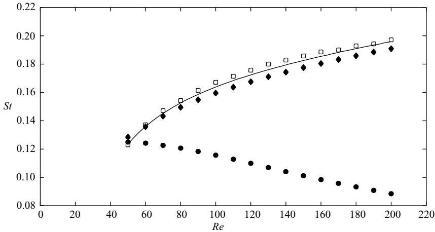
FIGURE 1. Evolution of the global selected frequency in the wake of a circular cylinder as a function of the Reynolds number. \square , Frequency obtained by direct numerical simulation (DNS); —, experimental results (from Williamson 1988). Results ( \omega_s ) represented by \blacklozenge have been obtained by applying the linear criterion \chi_s on the time-averaged mean flow. \bullet , The same calculation applied to the unperturbed basic flow. From Pier (2002)
